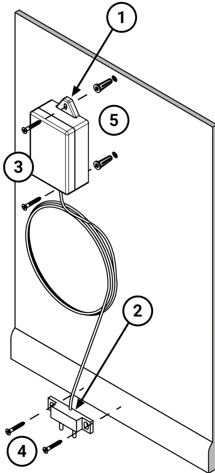
Figure 2: Drywall Installation
